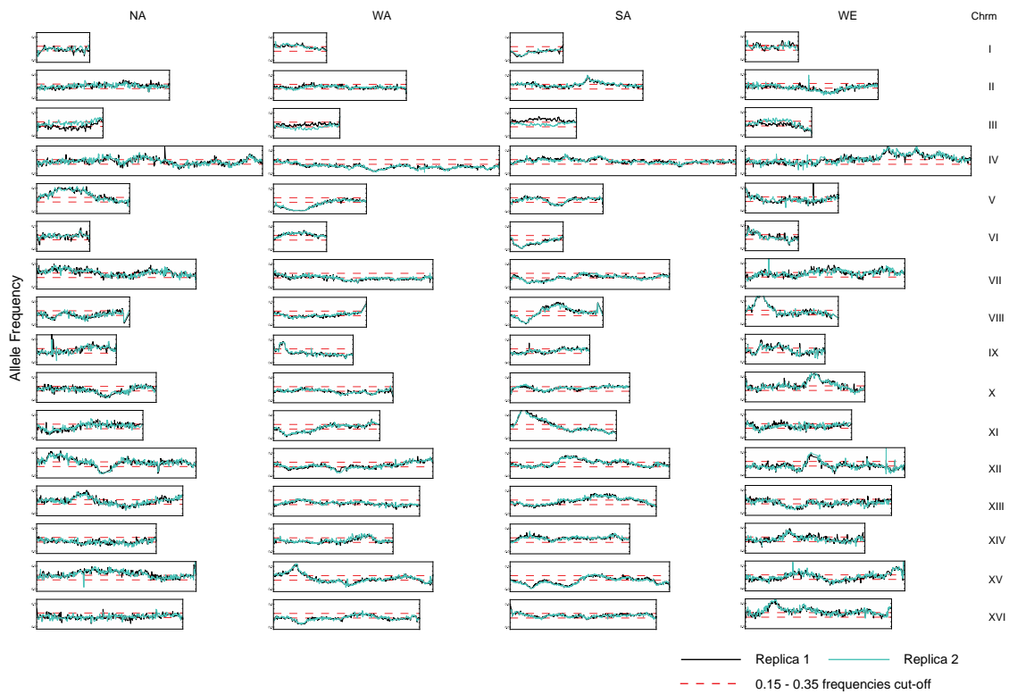
Figure S4 Genome-wide parental allele frequencies in the F12 SGRP-4X population. Allele frequencies for NA, WA, SA and WE parental strains are shown for each chromosome. Estimates were obtained for both replicas (black and light-blue lines) in haploid T4 mock samples. Dashed cut-off denotes regions with at least one parental allele frequency below 15% or above 35%.
