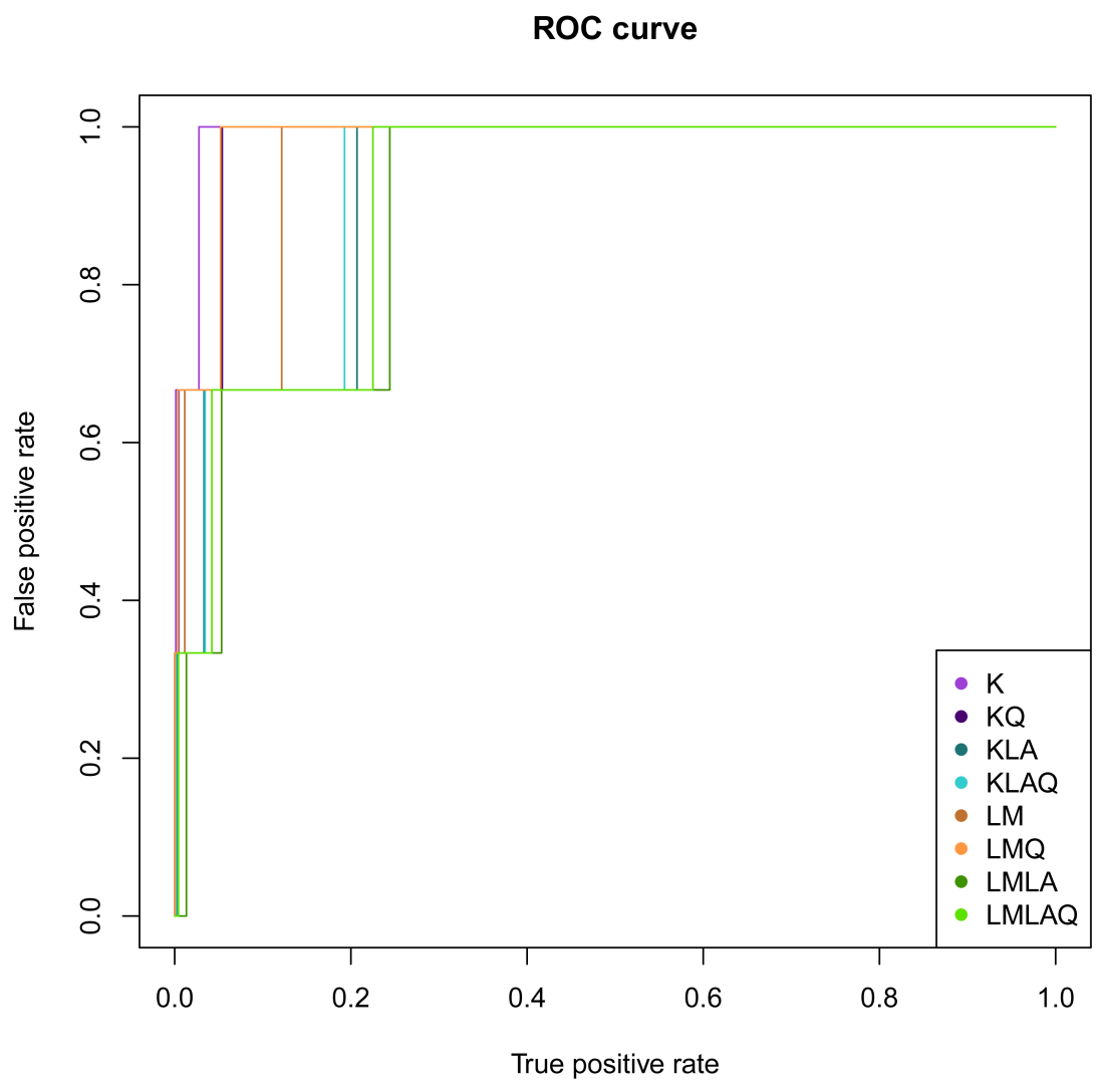
Figure S5 ROC curve of simulations with 3 causal SNPs each adding phenotypic value 10.
