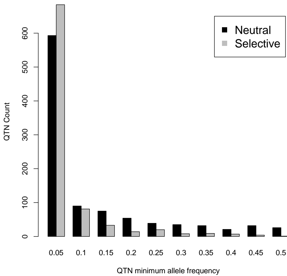
Fig. S1. Folded site frequency spectrum of QTNs in Large White for the two genetic architectures considered.
