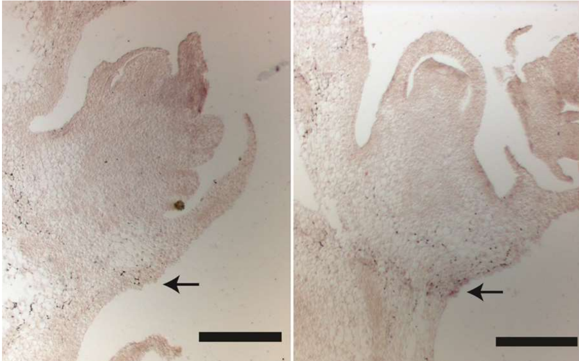
Figure S5. ZmYAB2.1 3'UTR probe hybridized to maize ears containing the maize allele (A) or the teosinte allele (B). Weak expression in the region homologous to the dehiscence zone (arrows) is only seen in in the teosinte allele (B). Scale bars are 200µm.
