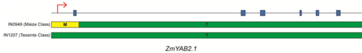
Figure S3. Cartoon showing recombination breakpoint of a RC-NIL (IN0949) in between Exon 1 and Exon 2 of ZmYAB2.1 . IN0949 carries maize regulatory region and mostly teosinte coding region, while IN1207 carries full teosinte regulatory and coding regions. IN0949 displays maize class ear internode length while IN1207 displays teosinte class ear internode length (Figure 1). IN0949 also has lower ZmYAB2.1 expression in comparison to IN1207 (Figure 2B).
