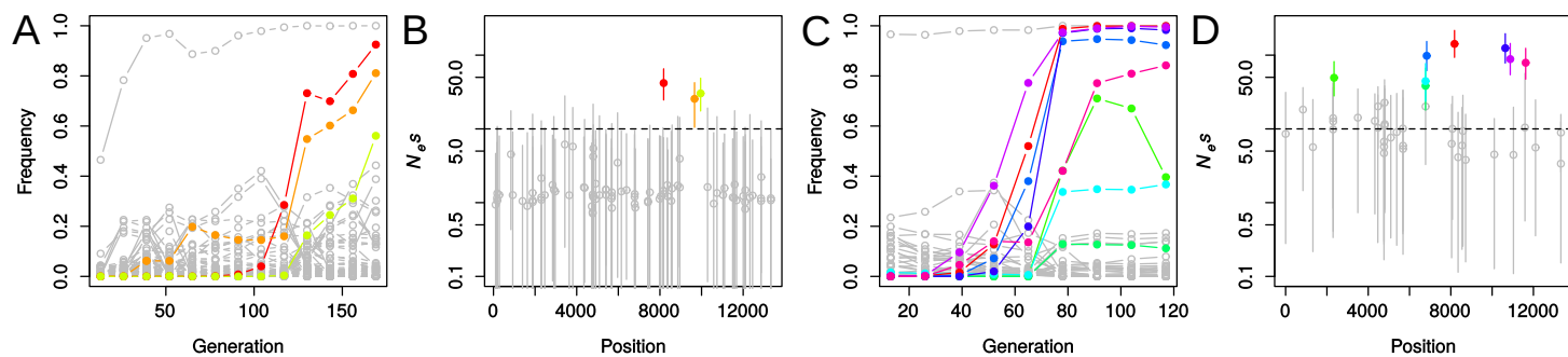
Figure S6: Allele trajectories (A, C) and posterior estimates for N_e s (B, D) for control (A, B) and drug-treated (C, D) Influenza. Non-significant loci are colored grey and significant loci are colored with a unique color for each locus.
