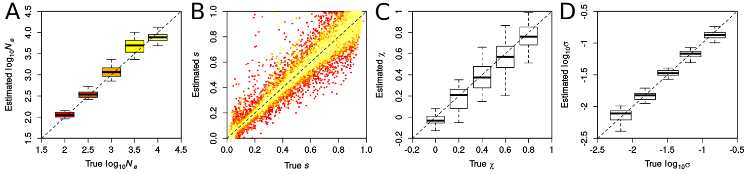
Figure S4: Accuracy in inferring demographic and selection parameters using the PLS 5/2 set of statistics. Results were obtained with ABC-PaSS using five and two PLS components for N_e and each s , respectively (PLS 5/2). Shown are the true versus estimated posterior medians for parameters N_e (A), s per locus (B), \chi and \sigma of the Generalized Pareto distribution (C and D, respectively). Boxplots summarize results from 25 replicate simulations, each with 100 loci. Uniform priors over the whole ranges shown were used. (A, B): N_e assumed in the simulations is represented as a color gradient of red (low N_e ) to yellow (high N_e ). (C,D): Parameters \mu and N_e were fixed to 0 and 10^3 , respectively, \log_{10}\sigma was fixed to -1 (C) and \chi was fixed to 0.5 (D).
