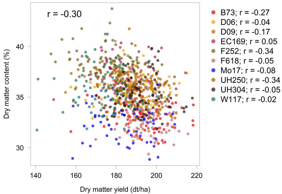
Figure S8 Scatterplot and phenotypic correlations between dry matter yield (dt/ha) and dry matter content (%) within each maize family (families are specified by their specific parental line).
