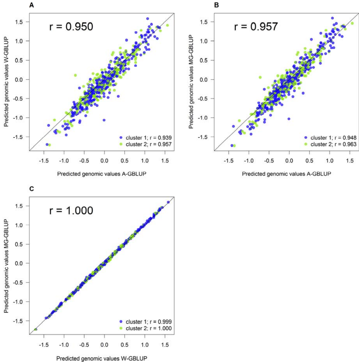
Figure S19 Comparison of predicted genomic values of wheat lines for environment 4 obtained from the three models. Colors indicate different wheat clusters. Overall correlations of predicted values as well as correlations within each cluster are given. A) Comparison of across group GBLUP (A-GBLUP) and within group GBLUP (W-GBLUP); B) Comparison of A-GBLUP and multi group GBLUP (MG-GBLUP); C) Comparison of W-GBLUP and MG-GBLUP.
