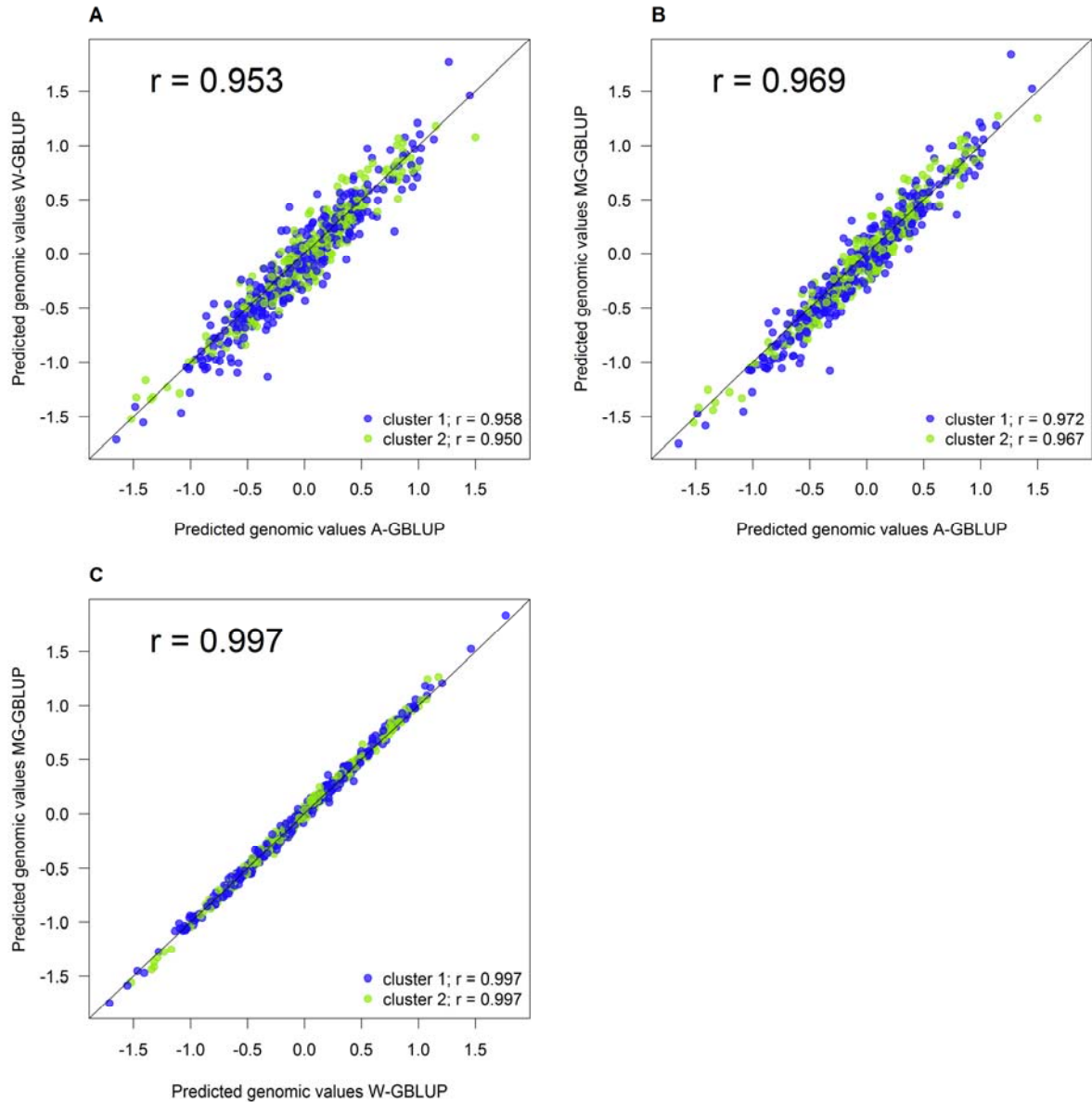
Figure S18 Comparison of predicted genomic values of wheat lines for environment 3 obtained from the three models. Colors indicate different wheat clusters. Overall correlations of predicted values as well as correlations within each cluster are given. A) Comparison of across group GBLUP (A-GBLUP) and within group GBLUP (W-GBLUP); B) Comparison of A-GBLUP and multi group GBLUP (MG-GBLUP); C) Comparison of W-GBLUP and MG-GBLUP.
