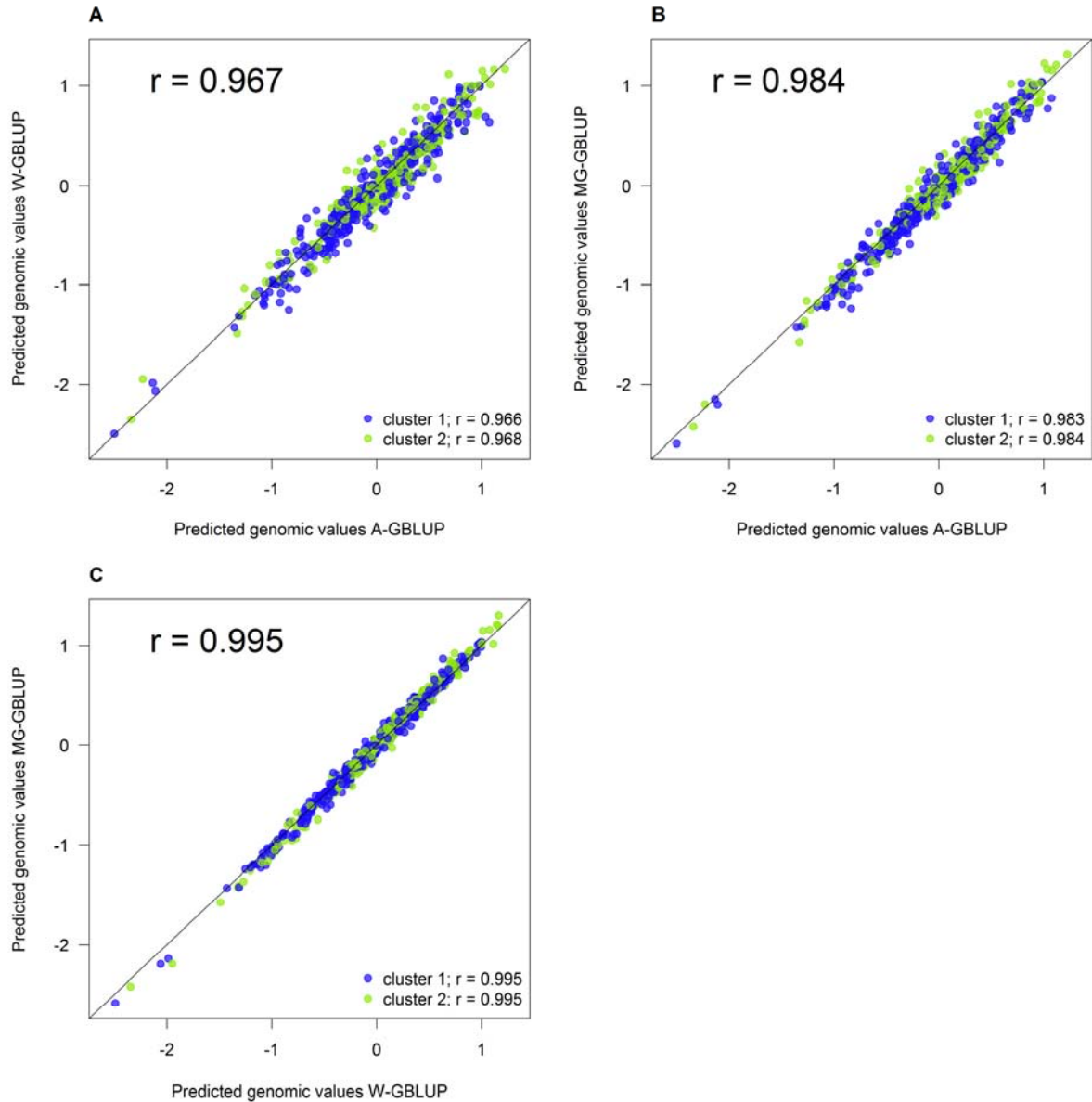
Figure S17 Comparison of predicted genomic values of wheat lines for environment 2 obtained from the three models. Colors indicate different wheat clusters. Overall correlations of predicted values as well as correlations within each cluster are given. A) Comparison of across group GBLUP (A-GBLUP) and within group GBLUP (W-GBLUP); B) Comparison of A-GBLUP and multi group GBLUP (MG-GBLUP); C) Comparison of W-GBLUP and MG-GBLUP.
