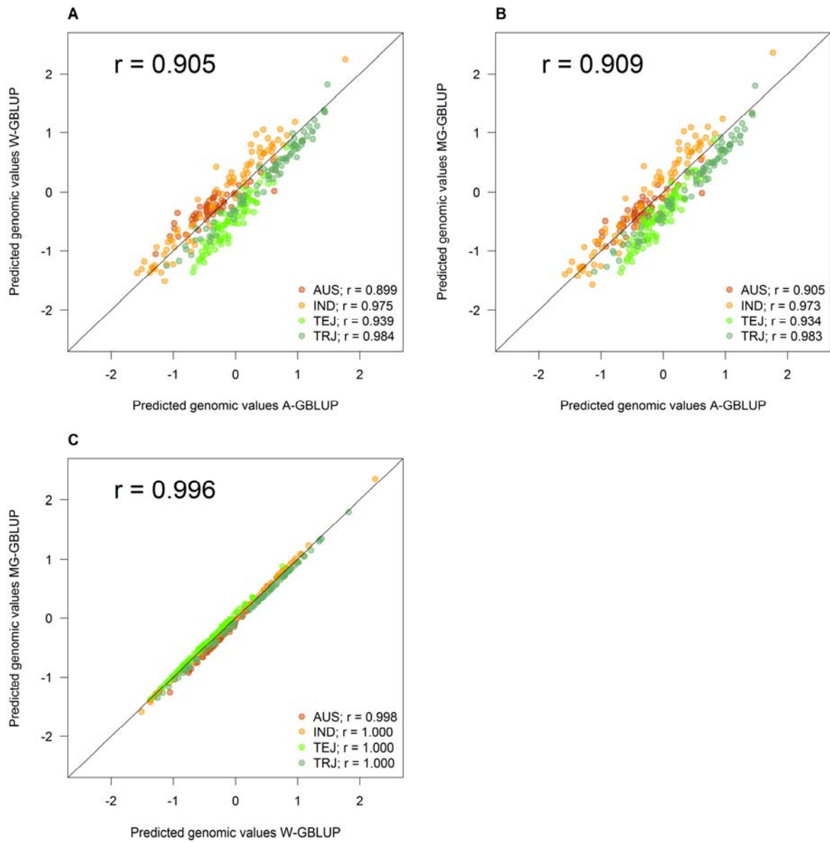
Figure S12 Comparison of predicted genomic values of rice lines for trait plant height obtained from the three models. Colors indicate different sub-populations (AUS, indica/IND, temperate japonica/TEJ, tropical japonica/TRJ). Overall correlations of predicted values as well as correlations within each sub-population are given. A) Comparison of across group GBLUP (A-GBLUP) and within group GBLUP (W-GBLUP); B) Comparison of A-GBLUP and multi group GBLUP (MG-GBLUP); C) Comparison of W-GBLUP and MG-GBLUP.
