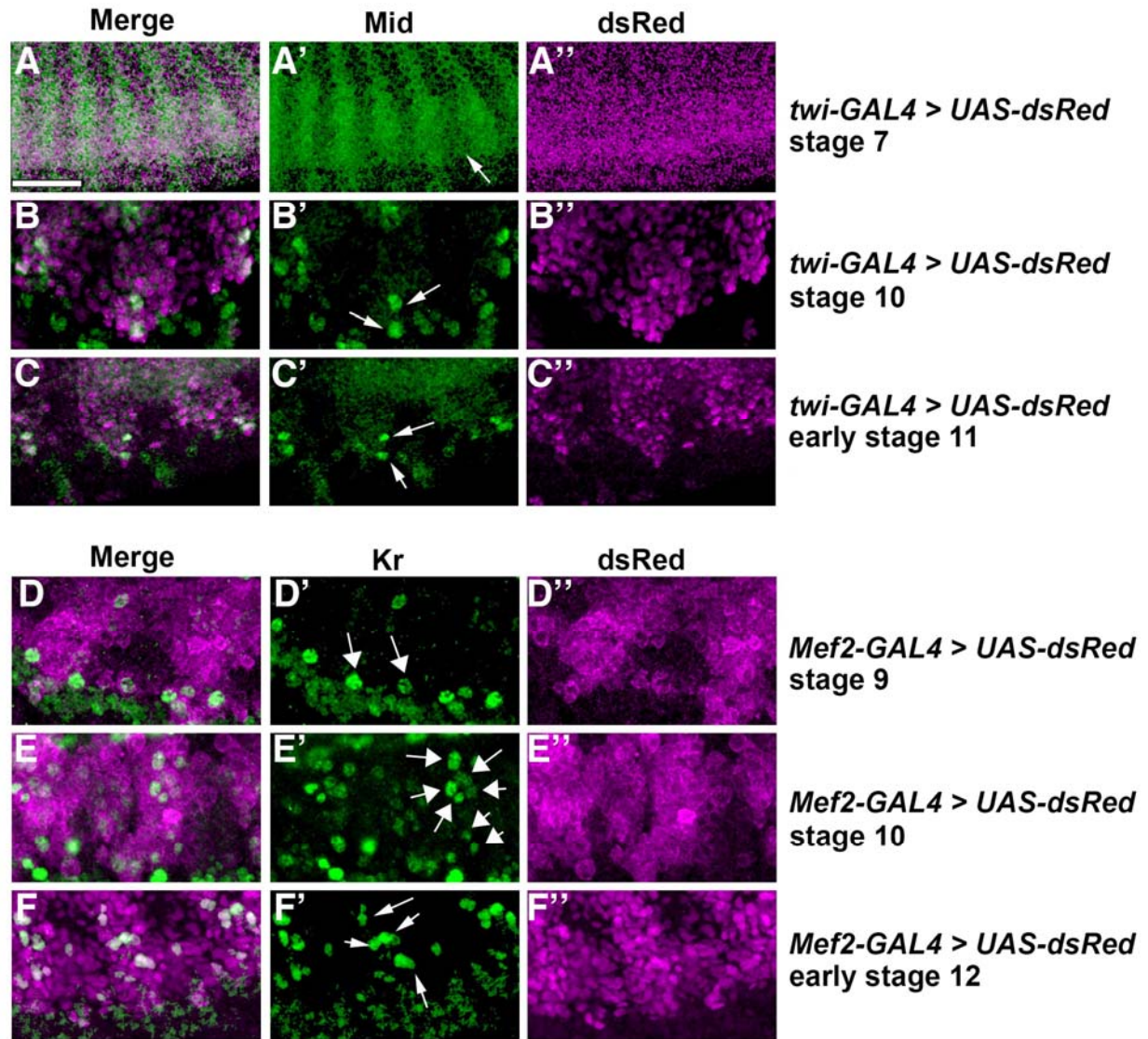
Figure S3 Expression of GAL4 lines used in this study. twi-GAL4 and Mef2-GAL4 are expressed during LT formation and development, and their expression overlaps with Mid. (A-A''') Panels show embryos in which twi-GAL4 drove a UAS-nuc::dsRed construct. Embryos were stained with anti-dsRed (magenta) and anti-Mid (green). Arrow points to co-expression at stage 7. (B-B''') twi-GAL4 > UAS-nuc::dsRed embryos at stage 10. Arrows point to the Mid-expressing progenitors. (C-C''') twi-GAL4 > UAS-nuc::dsRed embryos at early stage 11. Arrows point to the Mid-expressing progenitors. (D-D''') Mef2-GAL4 > UAS-nuc::dsRed embryos stained with anti-Kr (green) and anti-dsRed (magenta). Arrows point to Kr-expressing founders at late stage 11.
