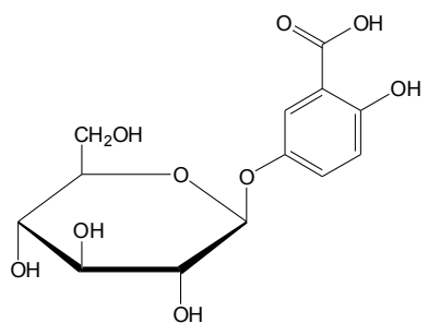
2,5-DHBAG
