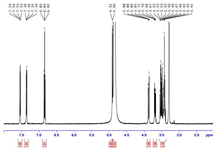
1 H NMR spectrum of compound 2
