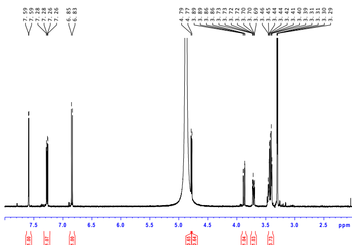
1 H NMR spectrum of compound 1
