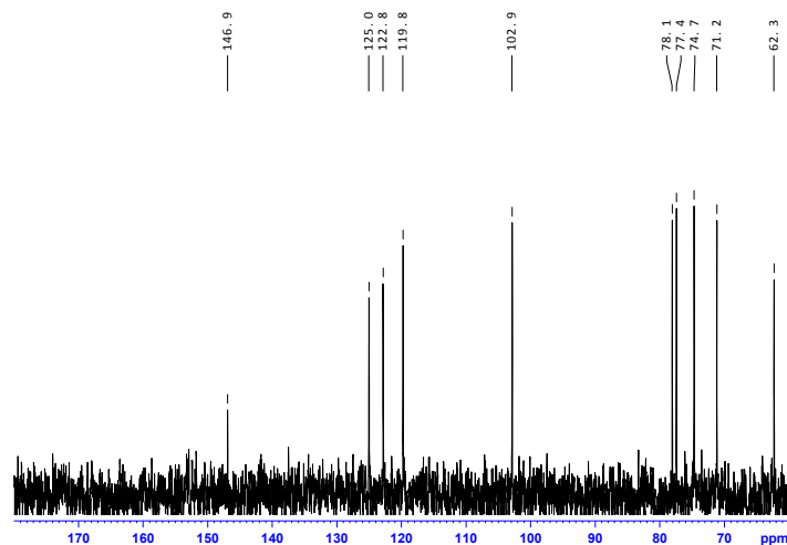
13 C NMR spectrum of compound 2
