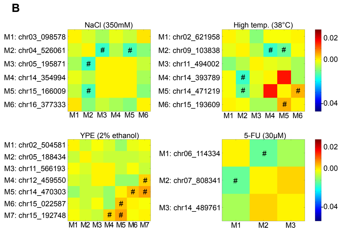
Figure S2: Interaction plots. (A) Heatmap of pairwise Interaction Distance (ID) between 1226 markers for high temperature phenotype (left panel). Blue points indicate strong synergistic effect between markers while red points indicate redundancy between markers (also seen in regions with high linkage). We focused on an interaction region between chr9 and chr14 by analysing it further with a denser markers set (977 and 479 respectively). The heatmap of this recalculated Interaction Distance is shown on the right panel. Several regions with low ID scores are seen (marked with *), suggesting the presence of additional interactions in this region, other than the confirmed
