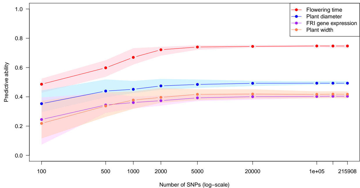
Figure S5 Predictive ability for marker subsets in the Arabidopsis data set. The predictive ability was estimated with fivefold cross-validation and 10 replications using RR-BLUP. Average predictive ability as a function of the number of randomly selected markers is visualized as a straight line for each trait. Shaded areas indicate the range of 10 different marker subsets.
