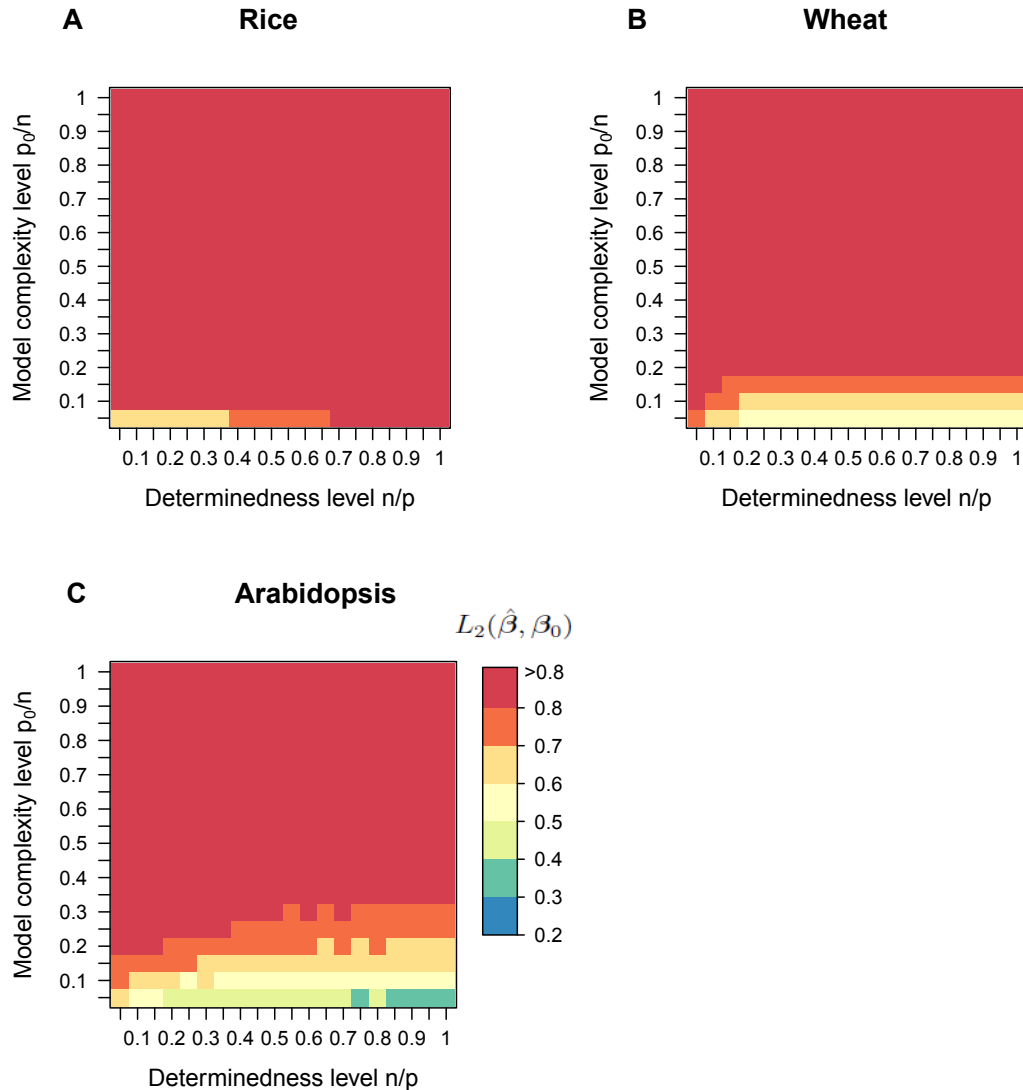
Figure S7 Heat maps for the normalized L_2 error of the elastic net with correlated predictor variables. The correlation structure of the simulated marker data was superimposed from the three experimental data sets (rice, wheat, and Arabidopsis ). The simulations were conducted according to procedure 3 (Figure S6). Each of the 400 scenarios ( p = 2,000 and h^2 = 0.75 ) was repeated 10 times and results were averaged over replications.
