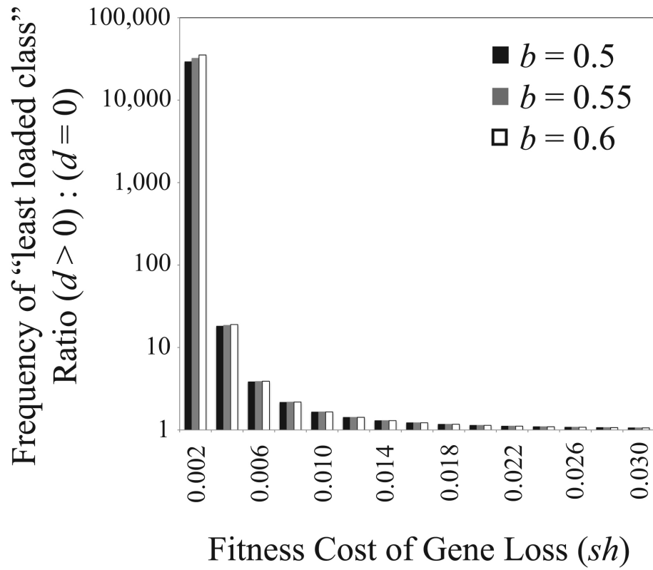
FIGURE S3.—Gene conversion increases the frequency of Y chromosomes haplotypes that carry zero deleterious mutations ( i.e. , the “least-loaded” genotypic class). Results use the same parameters as those of Fig. 3 with n = 50 , and with the biased gene conversion parameter ( b ) permitted to vary.
