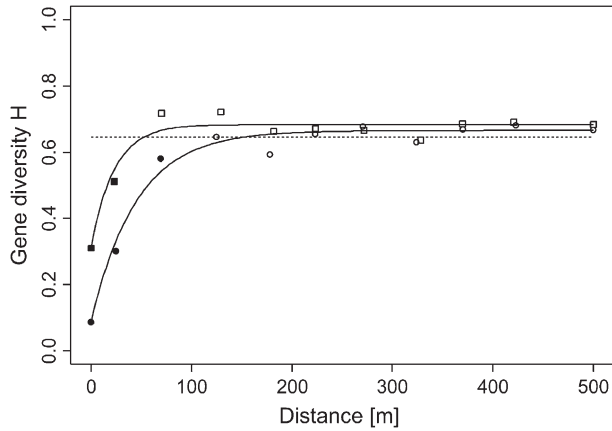
FIGURE 2.—Variogram of gene diversity \hat{H}(r) for a population of Lobaria pulmonaria . Each symbol denotes the mean semivariance over six microsatellite loci averaged over all pairs of thalli within each distance class. The semivariance is unweighted (circles) or weighted for recurrent genotypes (squares). The lines indicate the corresponding fitted exponential models; the dashed line shows the nonspatial model. Values below the dashed line correspond to positive, and values above the dashed line to negative, autocorrelation. Solid symbols indicate statistically significant positive autocorrelation based on a one-sided Mantel permutation test with progressive Bonferroni correction ( \alpha = 0.05 ).
