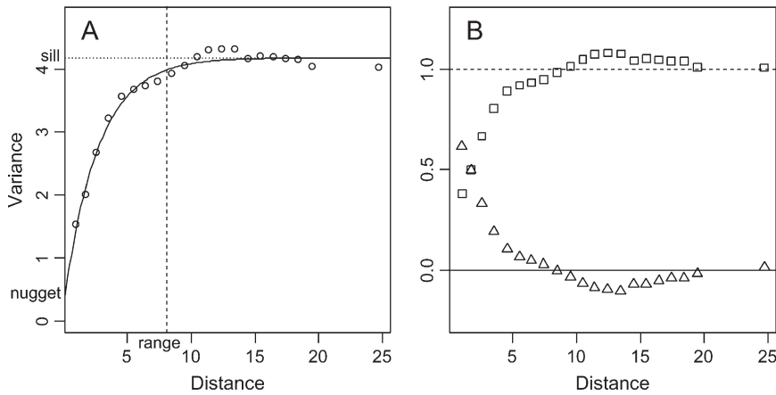
FIGURE 1.—Empirical variogram (A) and correlograms (B) for an artificial, spatially autocorrelated random variable simulated on a grid of 30 × 30 cells. Each symbol denotes the semivariance \gamma(r) (circles), Geary's c(r) (squares), or Moran's I(r) (triangles) calculated from all pairs of samples falling into each distance class r . The value for the last distance class of each series contains all pairs separated by >20 units and is drawn at the mean of the respective distances. (A) The solid line represents the fitted exponential variogram model. The dotted line (sill) indicates the population variance as estimated accounting for autocorrelation. The dashed line indicates the practical range, where the curve reaches
