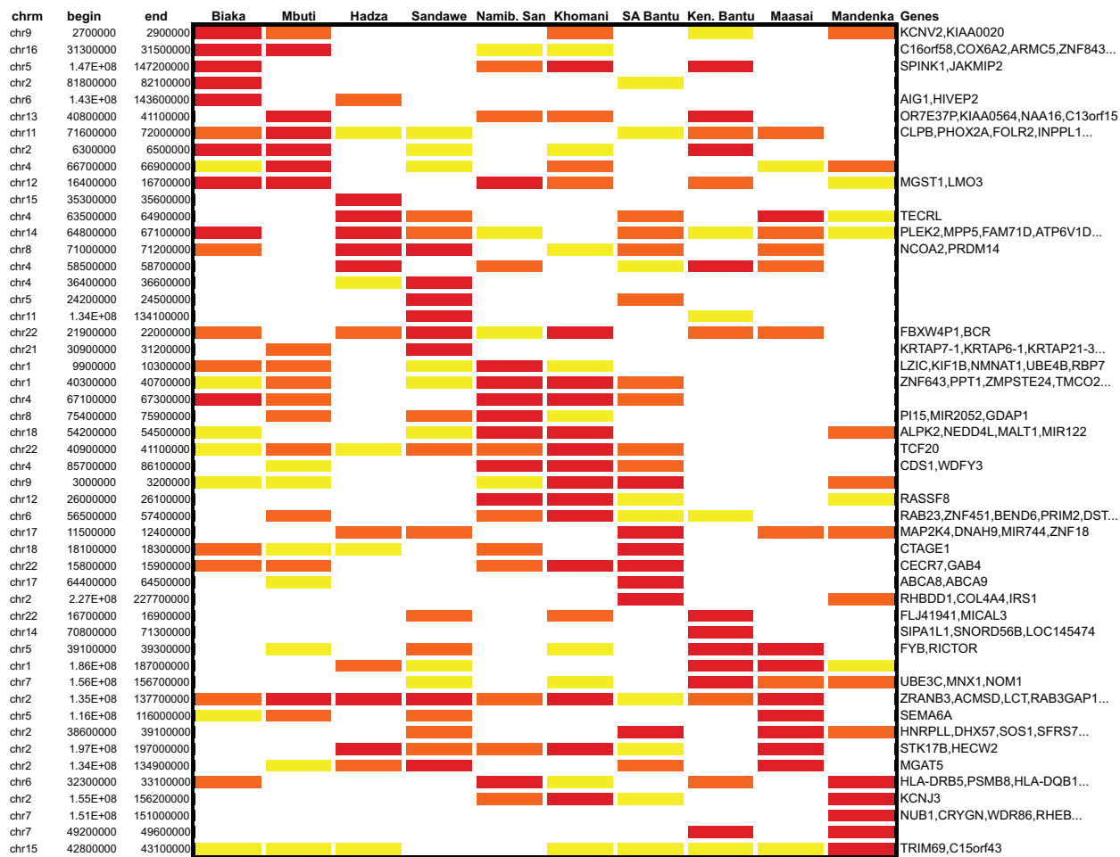
Figure S7. P-values for the 5 most extreme 100 kb genomic windows according to the XP-EHH YRI statistic in each population. Red indicates p < 0.01 , orange indicates p < 0.05 , yellow indicates p < 0.10 , and white indicates p > 0.10 . "Genes" column lists the genes located within the indicated windows.
