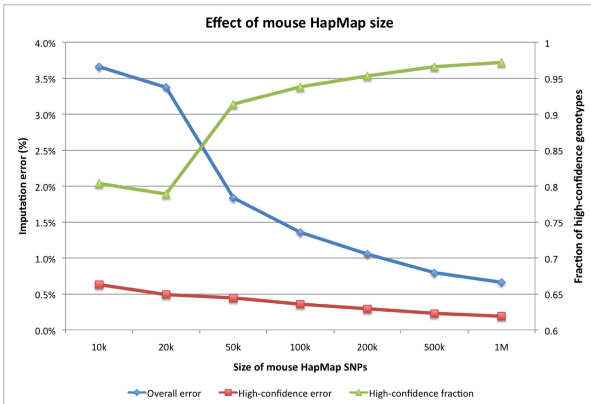
FIGURE S6.—Estimated imputation accuracy and coverage over fully-resequenced NIEHS/Perlegen SNPs across 12 classical inbred strains with various sizes of randomly selected SNP sets.
