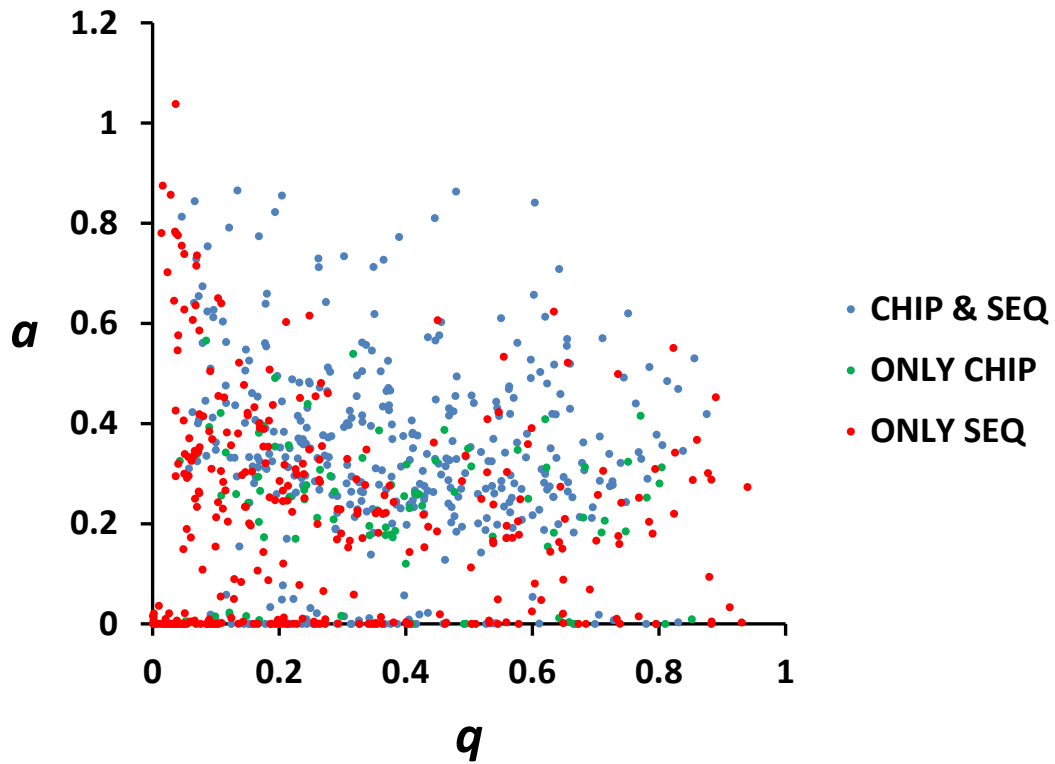
Figure S3. Joint distribution of effects on the trait ( a ; in phenotypic standard deviations) and frequencies ( q ) of all detected QTLs, separating those detected by the Chip analysis and Sequence analysis (blue), those detected only in the Chip analysis (green) and those detected only in the Sequence analysis (red). Results combining all genomes and values of \rho .
