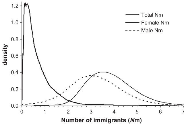
FIGURE 2.—Plots of the posterior densities of the number of immigrant genes ( Nm ) per deme per generation obtained from the analysis of five northwestern Swiss vole populations. The posterior density estimated using STRs is shown as a thin line, the posterior density estimated using mtDNA is shown as a thick line, and the estimated posterior density of the males obtained as a convolution of mtDNA and STR densities is shown as a dashed line.
