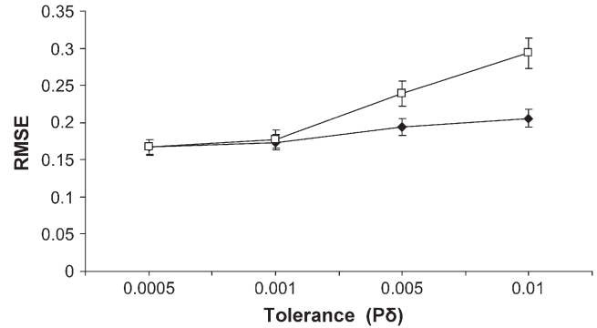
FIGURE 1.—A plot of RMSE for estimates of the migration parameter M vs. tolerance ( P_\delta ). Tolerance represents here the fraction of simulations retained for parameter estimation. Estimates using the standard ABC method are shown as open squares, and those using the modified weighted Euclidean distance are shown as solid diamonds. One million simulations were used for each estimation. Bootstrapped standard errors were calculated on 10,000 replicates and are reported here around point estimates.
