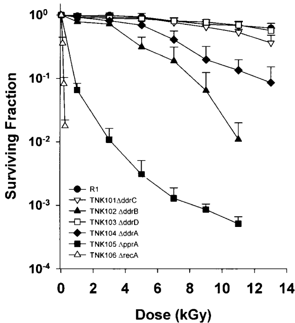
FIGURE 2.—Representative survival curves for D. radiodurans strains TNK101 \Delta ddrC , TNK102 \Delta ddrB , TNK103 \Delta ddrD , TNK104 \Delta ddrA , TNK105 \Delta pprA , TNK106 \Delta recA , and D. radiodurans R1 following exposure to \gamma -radiation. Values are the means \pm standard deviations of three independent experiments. n = 9 .
