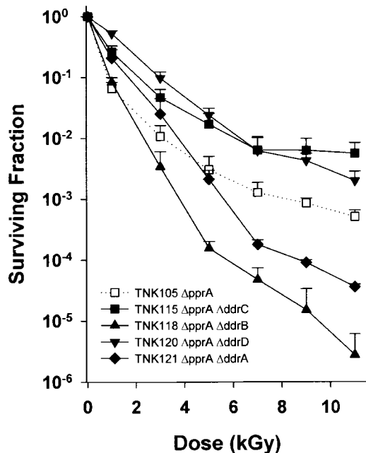
FIGURE 3.—Representative survival curves for D. radiodurans strains TNK105 \Delta pprA , TNK115 \Delta ddrC \Delta pprA , TNK118 \Delta ddrB \Delta pprA , TNK120 \Delta ddrD \Delta pprA , and TNK121 \Delta ddrA \Delta pprA following exposure to \gamma -radiation. Values are the means \pm standard deviations of three independent experiments. n = 9 .
