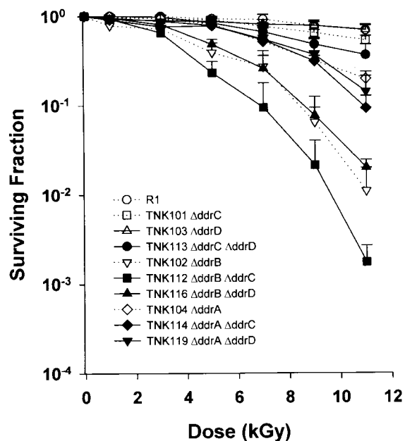
FIGURE 5.—Representative survival curves for D. radiodurans strains TNK112 \Delta ddrB \Delta ddrC , TNK113 \Delta ddrC \Delta ddrD , TNK114 \Delta ddrA \Delta ddrC , TNK116 \Delta ddrB \Delta ddrD , and TNK119 \Delta ddrA \Delta ddrD following exposure to \gamma -radiation. For comparison, the survival curves of TNK101 \Delta ddrC , TNK102 \Delta ddrB , TNK103 \Delta ddrD , TNK104 \Delta ddrA , and D. radiodurans R1 from Figure 1 are included as dotted lines. Values are the means \pm standard deviations of three independent experiments. n = 9 .
