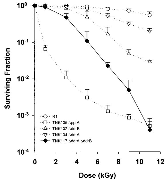
FIGURE 4.—Representative survival curve for D. radiodurans strain TNK117 \Delta ddrA \Delta ddrB . For comparison, the survival curves of TNK102 \Delta ddrB , TNK104 \Delta ddrA , TNK105 \Delta pprA , and D. radiodurans R1 from Figure 1 are included as dotted lines. Values are the means \pm standard deviations of three independent experiments. n = 9 .
