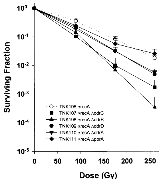
FIGURE 6.—Representative survival curves for D. radiodurans strains TNK106 \Delta recA , TNK107 \Delta ddrC \Delta recA , TNK108 \Delta ddrB \Delta recA , TNK109 \Delta ddrD \Delta recA , TNK110 \Delta ddrA \Delta recA , and TNK111 \Delta pprA \Delta recA following exposure to \gamma -radiation. Values are the means \pm standard deviations of three independent experiments. n = 9 .
