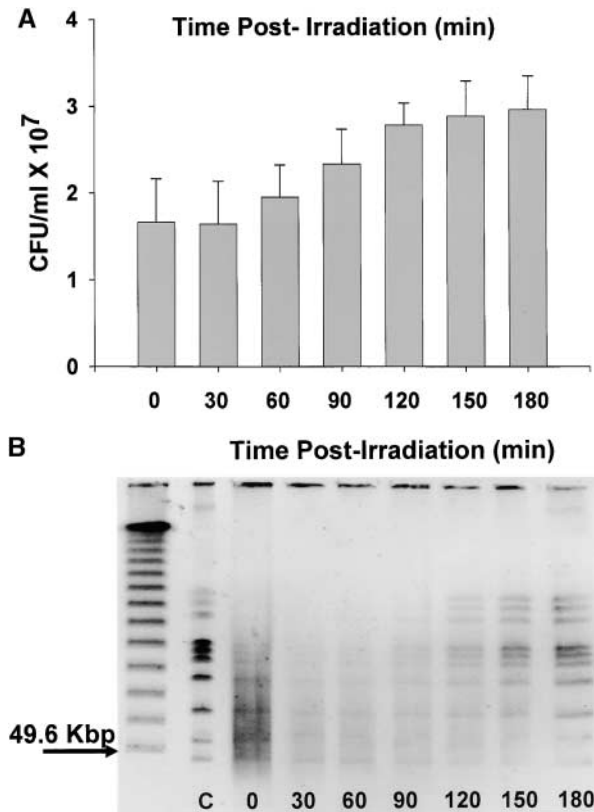
FIGURE 1.—(A) Growth of R1 cultures as a function of time following exposure to 3000 Gy \gamma -radiation. Titers were determined immediately after irradiation (zero time) and at the times indicated. (B) Pulsed-field gel illustrating the restitution of the R1 genome following 3000 Gy \gamma -radiation. The unlabeled lane corresponds to a lambda ladder standard. Lane C is a Not I digest of genomic DNA obtained from the culture prior to irradiation. The remaining lanes contain a Not I digest of genomic DNA isolated from irradiated cultures at the times indicated.
