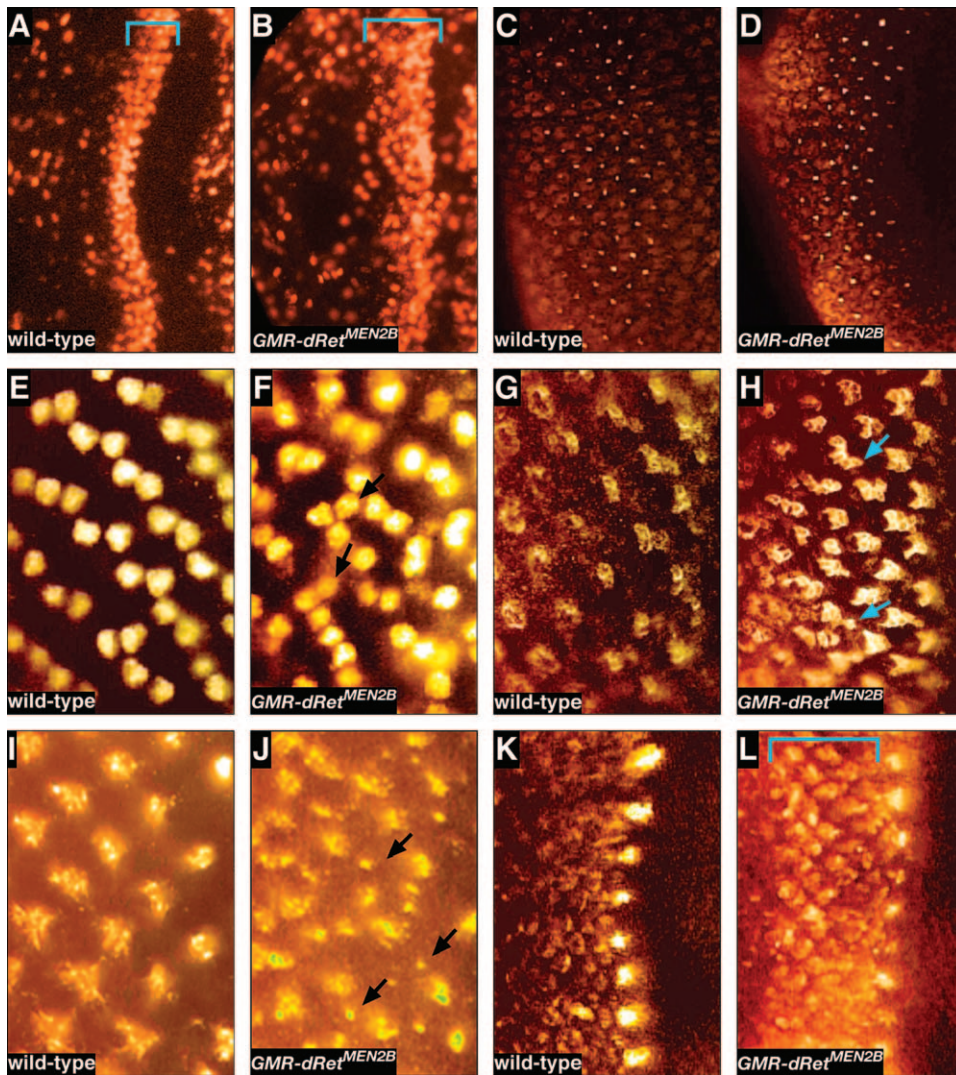
FIGURE 3. — GMR-dRet MEN2B directs excess proliferation, patterning defects, excess neuronal differentiation, and ectopic ERK activation. Anterior is toward the right. (A and B) The larval eye field differentiates in a posterior-to-anterior wave, and the brackets denote the second wave of mitoses; S-phase nuclei are visualized with BrdU (orange); note the ectopic S-phase cells in GMR-dRet MEN2B tissue. (C and D) Eye discs from GMR-dRet MEN2B flies (two copies) display a normal pattern of Boss staining (orange), indicating that early photoreceptor development (R8) is normal. Staining for Atonal (another marker for R8) in GMR-dRet MEN2B tissue is also normal (data not shown). These stains show that early development proceeds normally before GMR -driven dRet expression begins and that R8 retains its normal identity. (E and F) Eye discs from GMR-dRet MEN2B flies (two copies) contain disorganized Bar-expressing cells (arrows in F), suggesting aberrant recruitment, specification, or patterning of later-developing photoreceptor cells R1 and R6. (G and H) Eye tissue from GMR-dRet MEN2B flies (two copies) stained for Sev protein (orange) shows ectopic and aberrant clusters of Sev-expressing cells (arrows in H). Note that older, more posterior clusters of Sev-expressing cells are improperly spaced. (I and J) Photoreceptor neurons are visualized with 22C10, a neuronal-specific antibody. GMR-dRet MEN2B (two copies) eye tissue contains ectopic neurons (arrows in J) between abnormally spaced ommatidia containing variable numbers of neurons. (K and L) An antibody specific for activated, di-phospho-ERK protein indicated that GMR-dRet MEN2B (two copies) eye tissue contains high levels of activated ERK in irregular patches (bracket in L) posterior to the morphogenetic furrow after the onset of GMR -induced expression. Early di-phospho-ERK staining (anterior to bracket in L) is normal in GMR-dRet MEN2B discs prior to the onset of GMR -induced expression.
