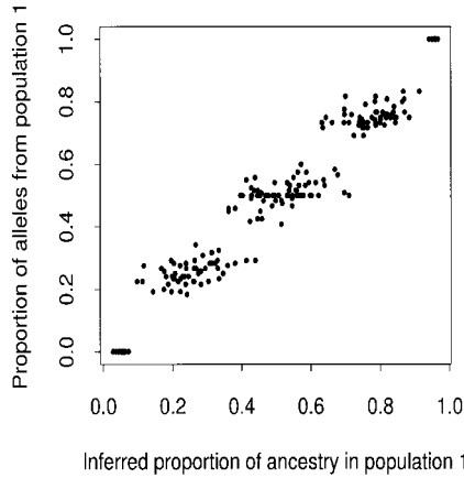
Figure 2.—Summary of the clustering results for simulated data set 3. Each point plots the estimated value of q_i^b (the proportion of ancestry in population 1) for a particular individual against the fraction of their alleles that were actually derived from population 1 (across the 60 loci genotyped). The five clusters (from left to right) are for individuals with 0, 1, . . . , 4 grandparents in population 1, respectively.
