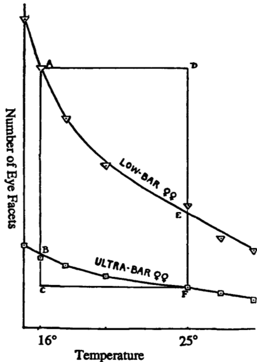
FIGURE 1.—Modified from HOGBEN (1933a, p. 384). The graphs, as indicated, are for the low-Bar and ultra-Bar genotypes. Ordinate, number of eye facets; abscissa, temperature during development. The data are from KRAFKA (1920). For a full discussion, see the text.
