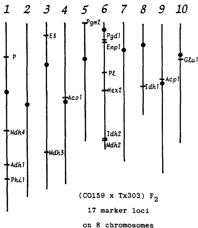
FIGURE 1.—Distributions of the 20 and 17 marker loci segregating in the F 2 populations: T232 × CM37 and CO159 × Tx303, respectively.
